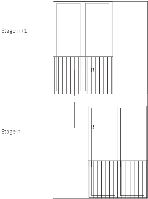
Facade 1:50
